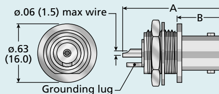
Figure 6 (Isolated Ground)
