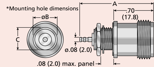
Figure 4 (Front Mount, Turret Contact)
