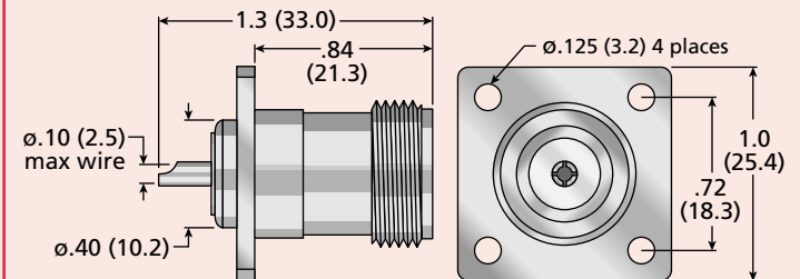
Figure 6 (Straight Panel Jack)
