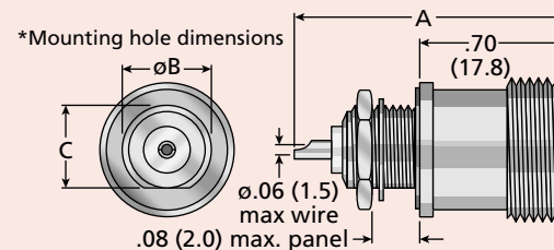
Figure 3 (Front Mount, Solder Pot Contact)
