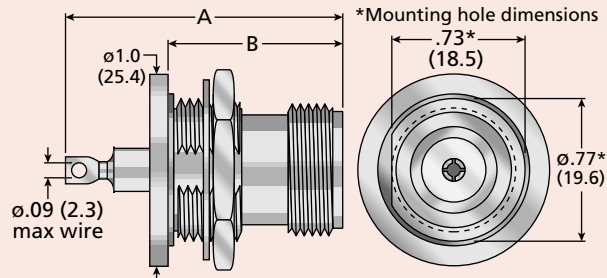
Figure 2 (Rear Mount, Flattened & Pierced Contact)
