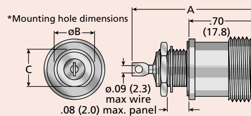
(Front Mount, Flattened & Pierced Contact)
