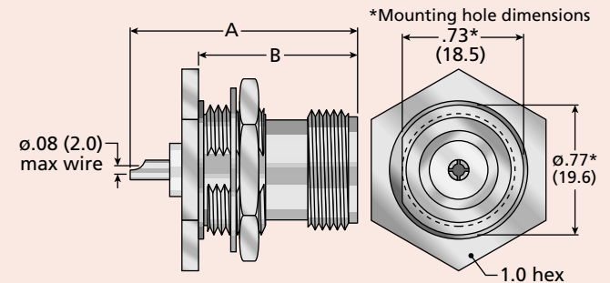
Figure 1 (Rear Mount, Solder Pot Contact)
