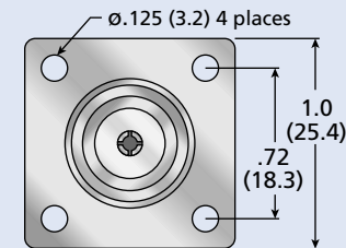
Front View Typical
