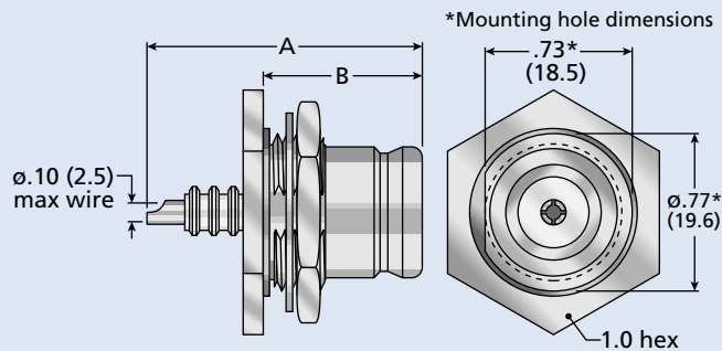
Figure 2 (Rear Mount, Solder Pot Contact High Voltage)
