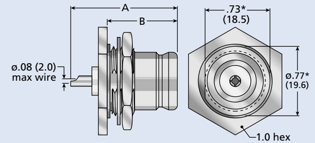
Figure 1 (Rear Mount, Solder Pot Contact)
