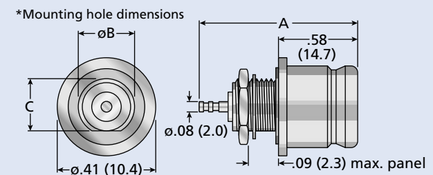
Figure 4 (Front Mount, Turret Contact)
