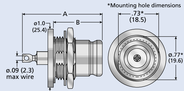
Figure 3 (Rear Mount, Flattened & Pierced Contact)
